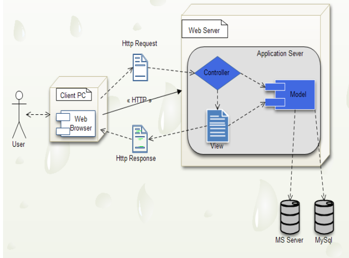
Figure 3. Mulungushi University SIS System Architecture
