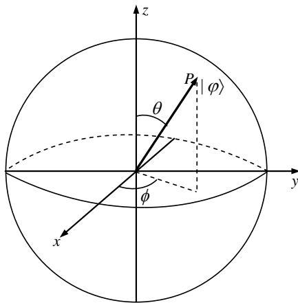
Figure 1. A qubit description on the Bloch sphere
