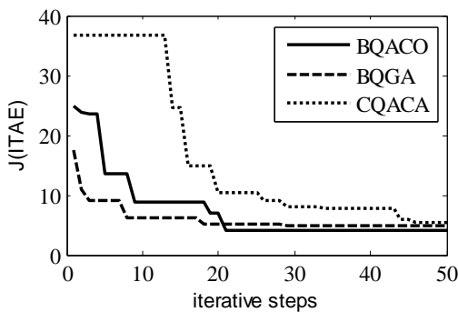
Figure 3. ITAE integral index comparison
