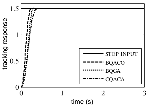
Figure 4. Tracking response curve comparisons of Fuzzy controllers
