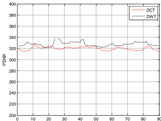
Figure 6. PSNR of the transferred packets
