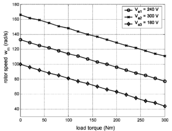
Figure 5 Torque-speed characteristics for three different armature voltages.
