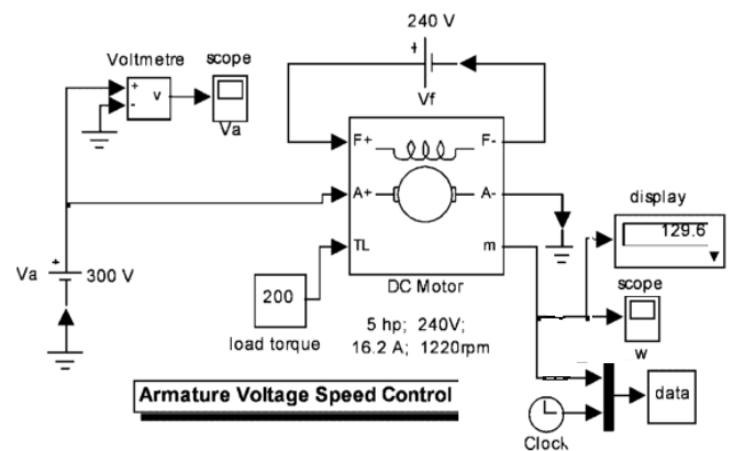
Figure 2 Simulink implementation of armature voltage speed control method.
