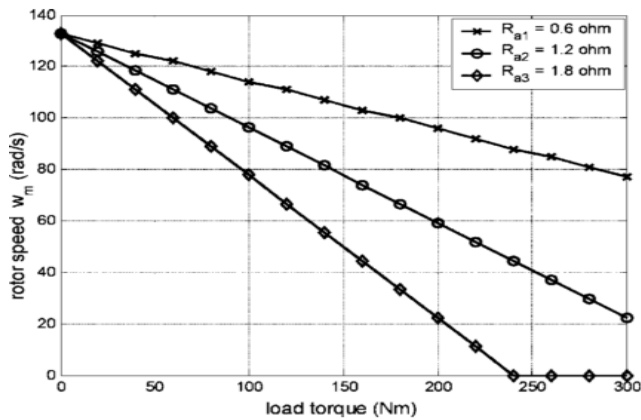
Figure 6 Torque-speed characteristics for three different resistances.
