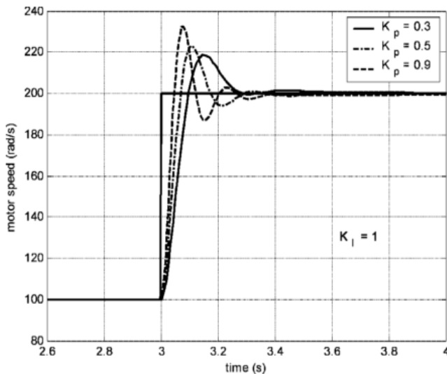
Figure 7 Motor speed for different PI gain values.
