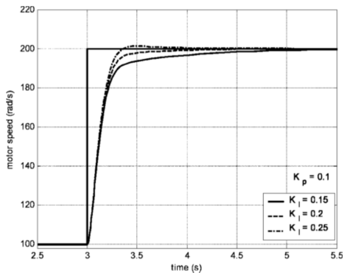
Figure 9 Motor speed for different PI gain values.
