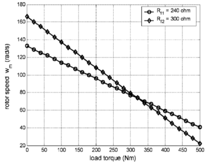
Figure 4 Torque-speed characteristics for two different field resistances.
